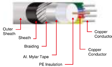
Cross Section View for 3+1 CCTV
